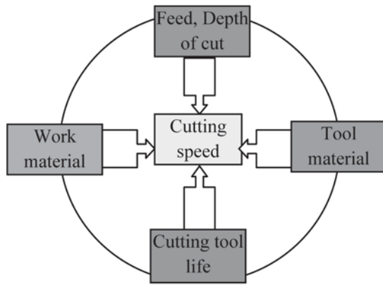
Figure 9. The factors significantly influencing cutting speed.
