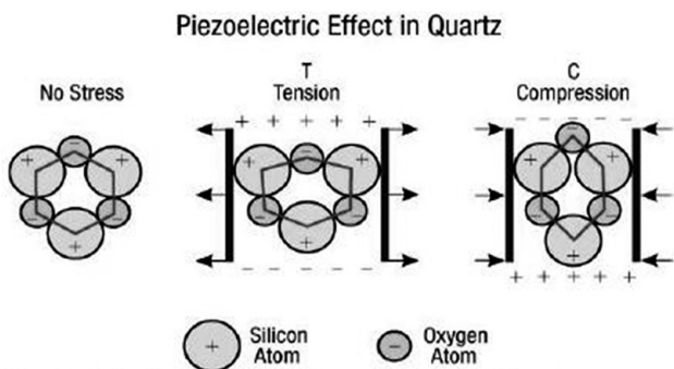
Figure 2. Mechanism of piezoelectric effect in quartz crystal.
