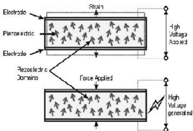
Figure 1. Conversion of Mechanical Energy into Electric Energy and vice-versa.
