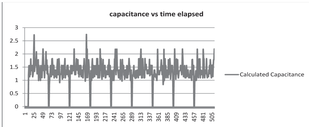
Figure 4. Plot of Capacitance vs Testing time(s).
