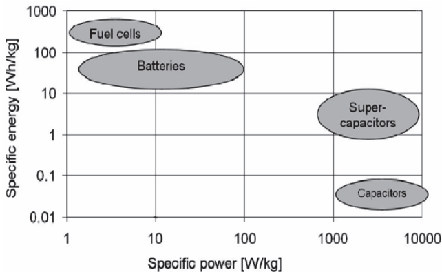
Figure1: Ragone plot of energy storage devices [3].
