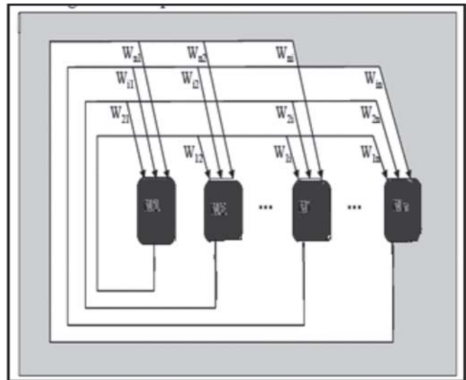
Figure 1. Hopfield Neural Network.
