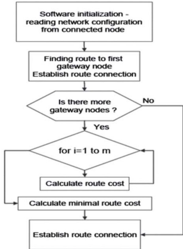
Figure 3. Proposed Routing Algorithm.
