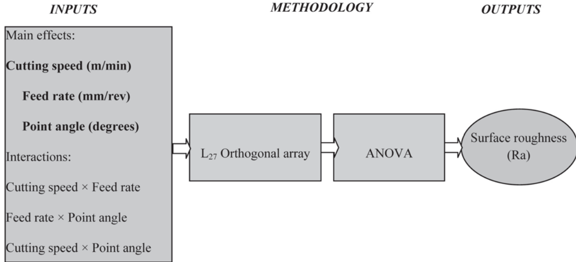
Figure 4. Flow diagram of methodology for analysis of surface roughness (Ra) in drilling [2].
