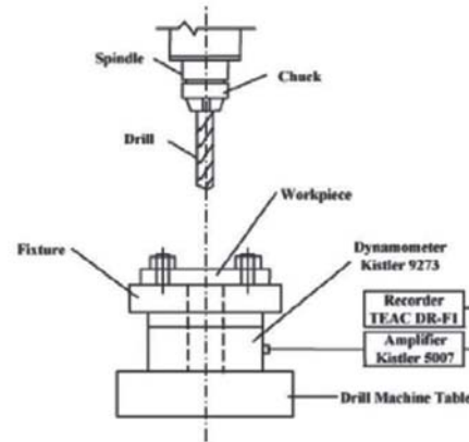
Figure 6. Line diagram of experimental set-up [3].
