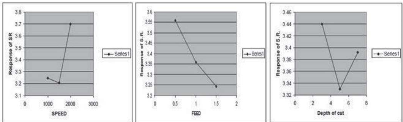
Figure 8. Effects of parameters on surface roughness [3].
