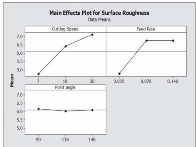
Figure 5. AOM plots indicating the effect of drilling parameters on surface roughness [2].
