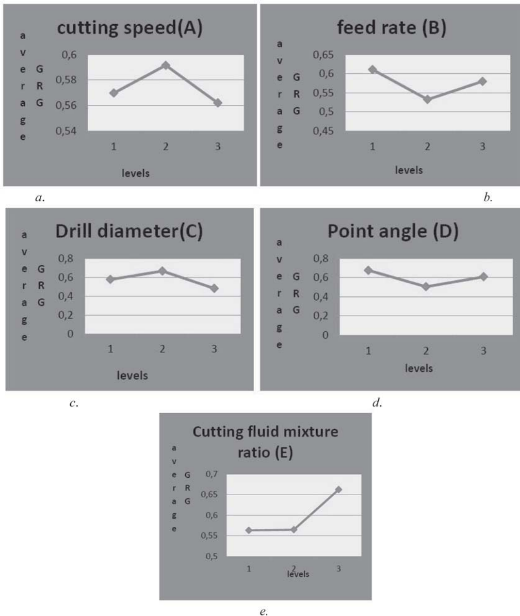
Figure 3. a-e: Graphs of grey relational grade for individual drilling parameters [1].
