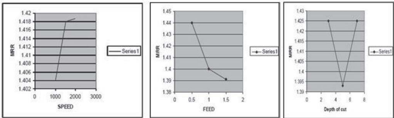
Figure 7. Effects of parameters on MRR [3].
