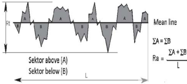
Figure 11. Definition of the mean line in evaluation of surface roughness.
